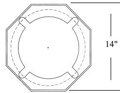
(4) 3/4" ANCHOR BOLTS ON A 12" DIA. BOLT CIRCLE
