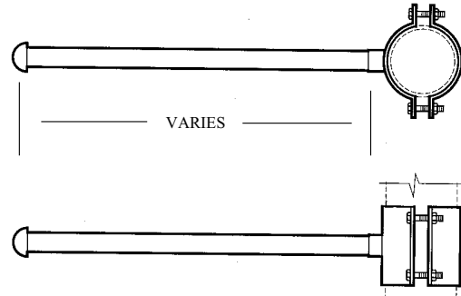
CLAMP ON MOUNTING
