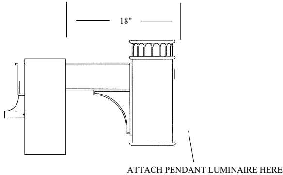
POLE SIDE MOUNT CLAMP TYPE
