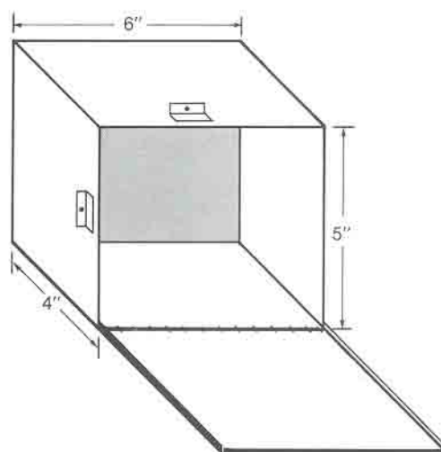
WALLPACK JUNCTION BOX 4" x 6" x 5"
